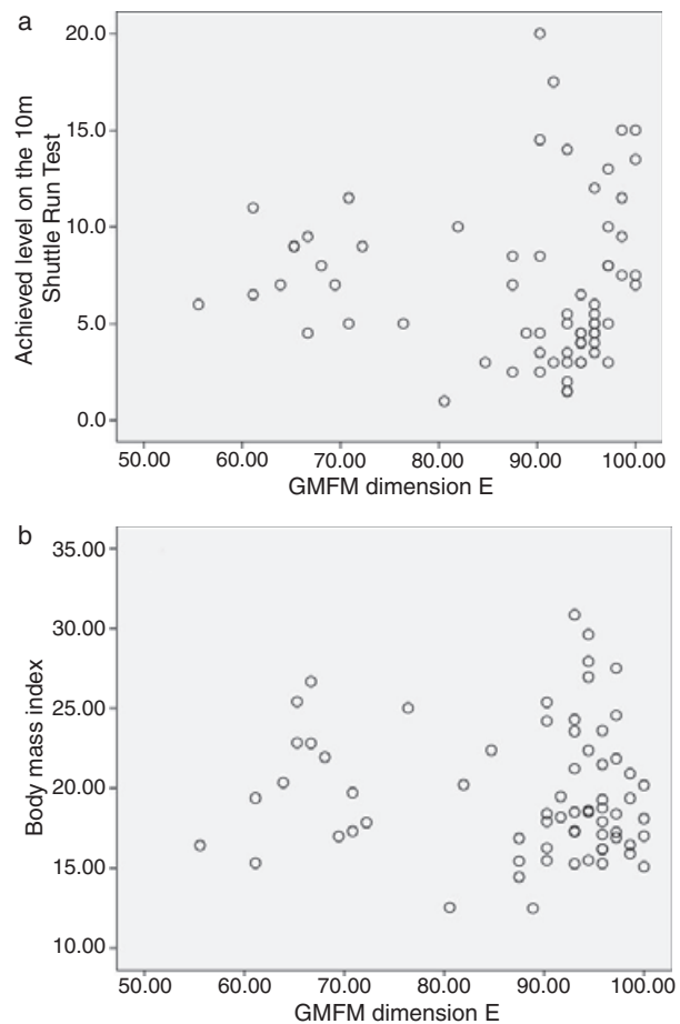
Figure 1: A scatterplot showing the relationship between (a) aerobic capacity and (b) BMI and gross motor capacity (Gross Motor Function Measure, dimension E).
